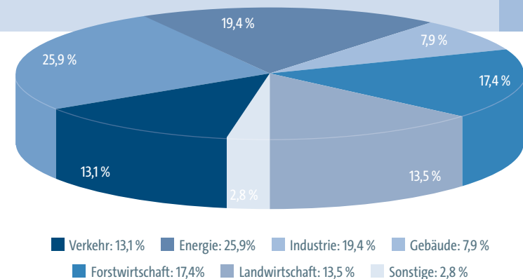
Kyoto-Emissionen weltweit (2004) (CO 2 | Methan | N 2 O | FCKW/FKW | SF 6 )
